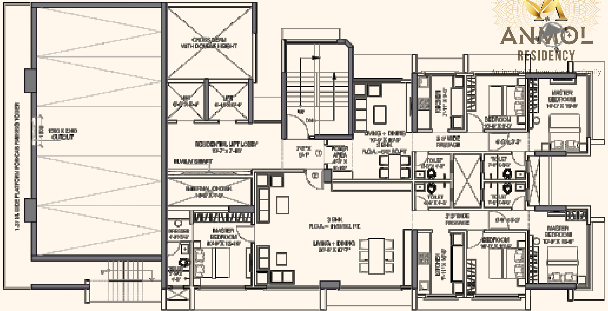
7TH TO 10TH FLOOR PLAN
